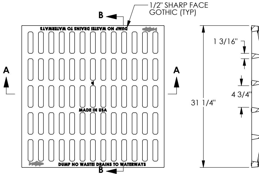
SECTION B-B
